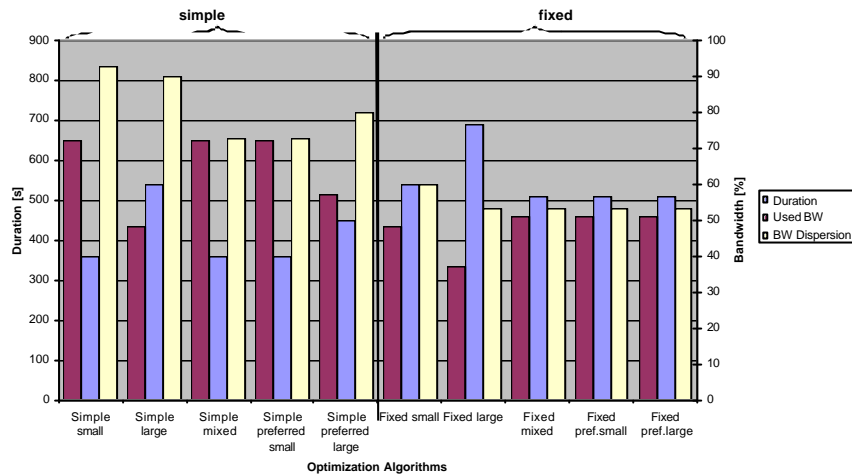
Figure 10: Comparison of simple/fixed optimization, BW limit = 3000kbps
