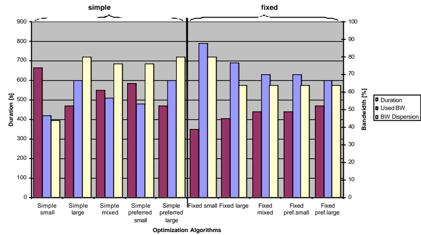
Figure 9: Comparison of simple/fixed optimization, BW limit = 2500kbps
