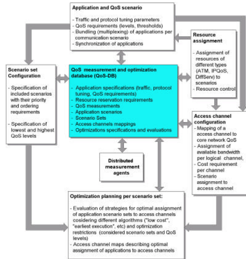
Figure 2: Components of QORE
