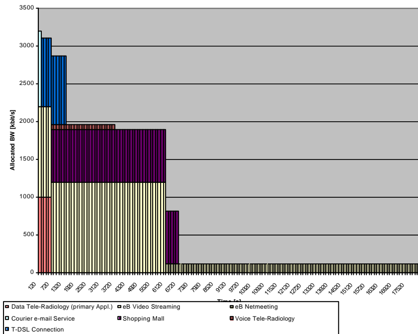
Figure 6: QORE optimization using the „Mixed Bandwidth“ algorithm
