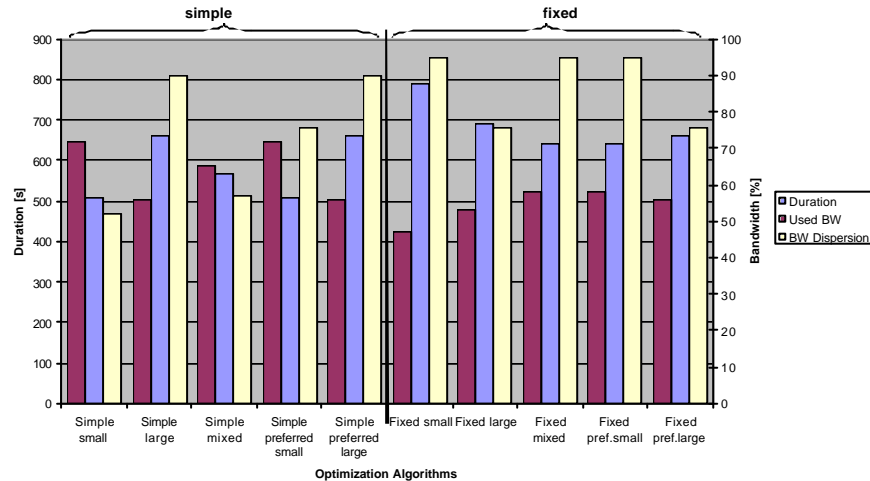
Figure 8: Comparison of simple/fixed optimization, BW limit = 2100kbps
